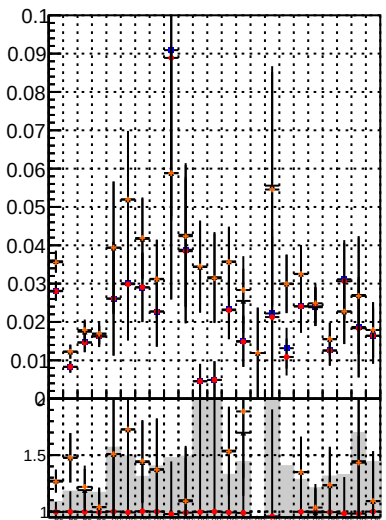
Fake rate vs. BQM, BQMS, PLMS, PixelLessOrandom mod MS
