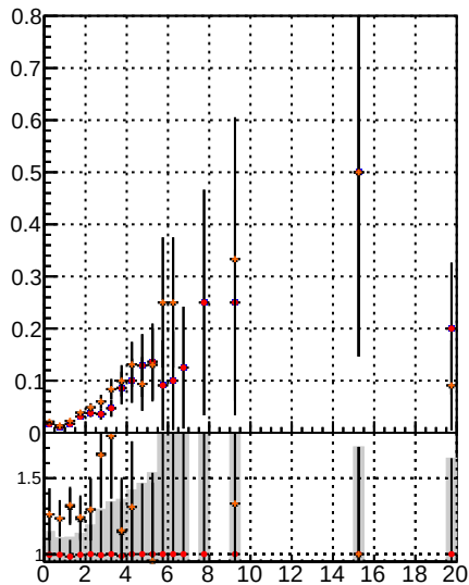
Fake rate vs. BQM, BQMS, PLMS, PixelLessOrandom mod MS
