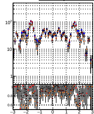
N of reco track vs \eta BQM RMS PL pixelLess BQM mod MS
