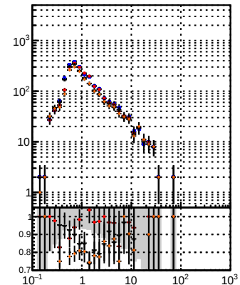
N of reco track vs \eta BQM RMS PL pixelLess BQM mod MS
