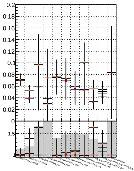
Fake rate vs. BQM, noMS, PLMS, PixelLessOrNoBQM mod MS
