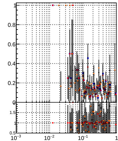
Fake rate vs \mu Legend: DOM noMS DOM MS PL Orig/DOM orig MS pixelLessOrig/DOM mod MS
