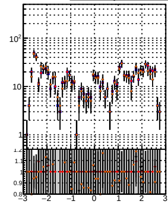
BSM MS PL pixelLess N of reco track vs \eta BSM mod MS
