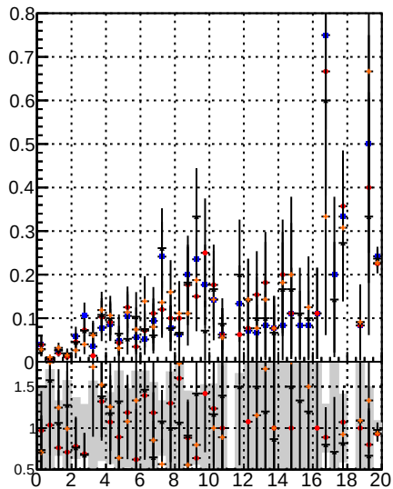
Fake rate vs. BQM noMS BQM noMS, PLMS BQM noMS, PLMS PixelLess or noBQM mod MS
