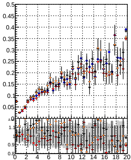
Fake rate vs. BQM, noMS BQM, noMS, PL pixelLessOrNoDOM mod MS
