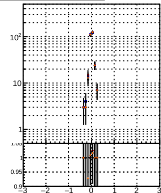
BGM RMS MS PL pixelLess N of associated (recoToSim) tracks vs \eta
