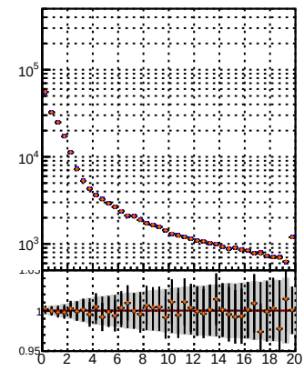
N of reco track vs. \chi^2 BQM reMS BQM reMS PL BQM reMS PL MS pixelLess or random mod MS
