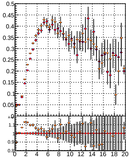
Fake rate vs. \chi^2 Legend: Blue line: BQM noMS Red line: BQM noMS PLMS Orange line: BQM noMS PLMS mod MS Grey shaded area: Difference from nominal
