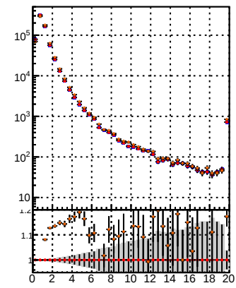
N of reco track vs. \chi^2 BQM RMS PL MS pixelLess random mod MS
