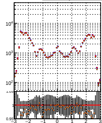
BSM, MS, PL, pixelLess, BSM mod MS N of reco track vs \eta
