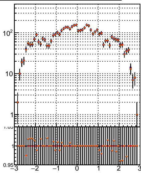
N of simulated tracks vs phi —•— DQM_noMS —♦— DQM_noMS_PL —▲— Orig/DQM_orig_MS —▼— pixelLessOrig/DQM_mod_MS
