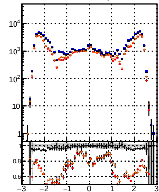
N of reco track vs \eta BGM RMS PL pixelLess RMS BGM mod MS
