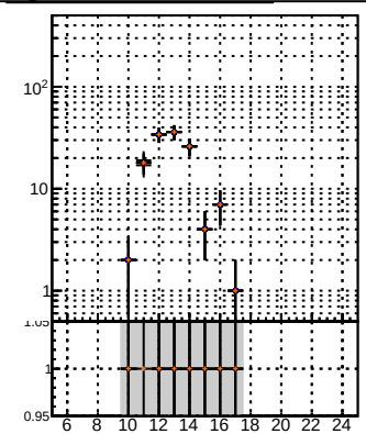
N of reco track vs hit DOM no MS DOM mod MS orig DOM orig MS pixelLessOrig/DOM mod MS
