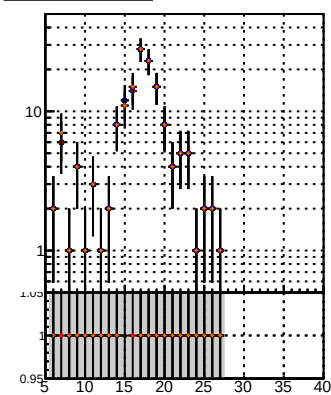
N of reco track vs hit DOM no MS DOM mod MS orig DOM orig MS pixelLessOrig/DOM mod MS
