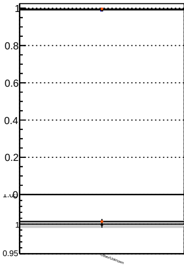
Fake rate vs. \chi^2
