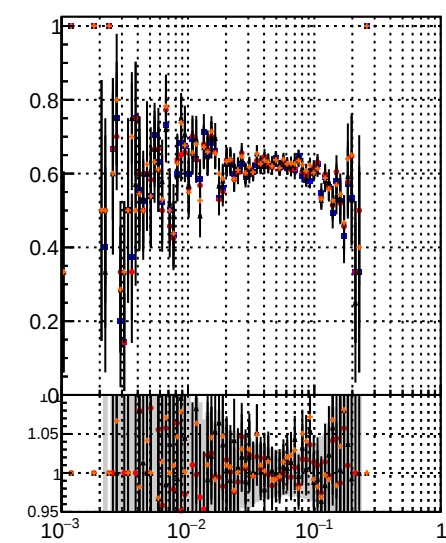
Fake rate vs dr Legend: DOM noMS (black line with dots) DOM MS PL (blue line with dots) orig/DOM orig MS (red line with dots) pixelLessOrig/DOM mod MS (orange line with dots)
