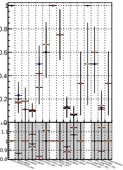
Fake rate vs. BQM, pMS, PL, pixelLessOrandom mod MS
