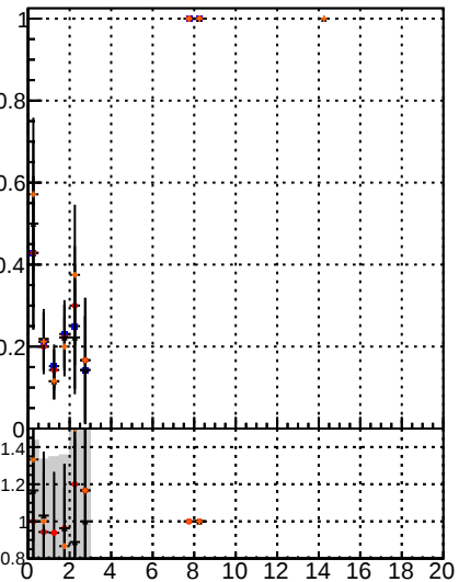
Fake rate vs. BQM, pMS, PL, pixelLessOrandom mod MS
