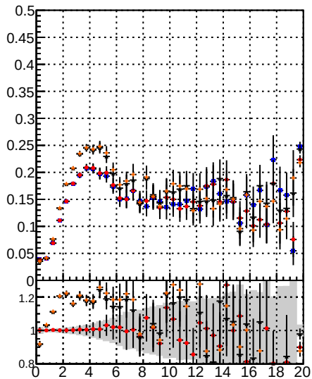
Fake rate vs. BGM p0MS PLMS pixelLessOrIdBGM mod MS
