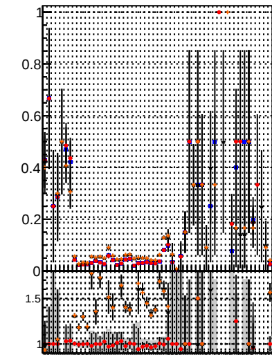
Fake rate vs. BGM noMS PLMS pixelLessOrNoBGM mod MS
