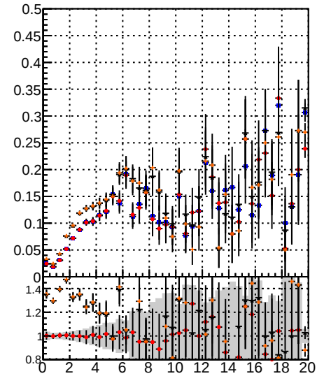
Fake rate vs. BGM noMS PLMS pixelLessOrNoBGM mod MS
