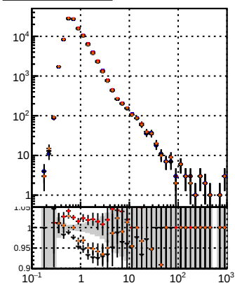
BGM RMS MS PL pixelLess N of reco track vs \eta
