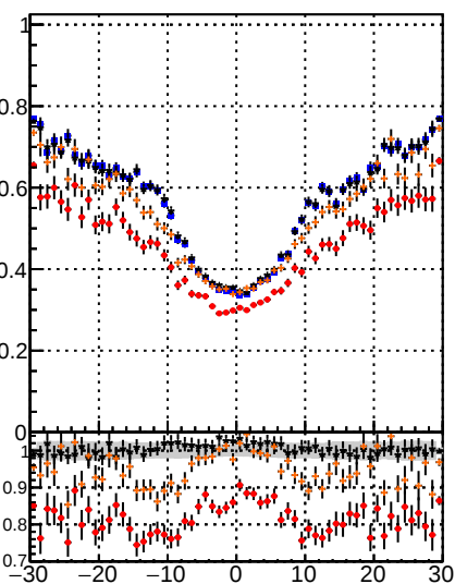
Fake rate vs d BQM pTMS PLMS pixelLessOrBQM mod MS
