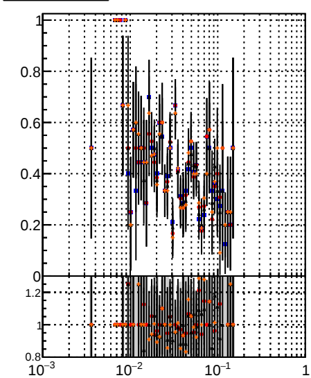
Fake rate vs dr Legend: DOM noMS (black line) DOM MS PL (blue line) Orig/DOM orig MS (red line) pixelLessOrig/DOM mod MS (orange line)
