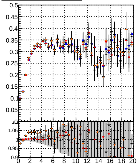
Fake rate vs. BQM, BQMS, PLMS, PixelLessOrigiDOM mod MS
