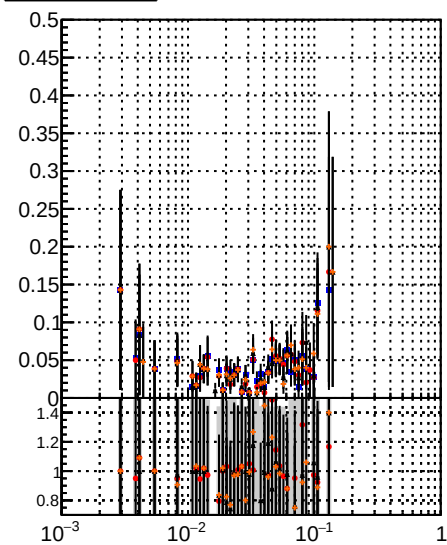
Fake rate vs \frac{\text{pixelLessOrig}}{\text{DOM mod MS}}
