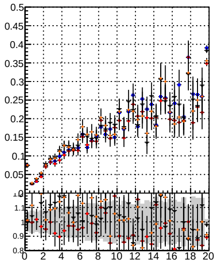
Fake rate vs. BSM, BSMs, PLMS, PixelLessOrIDOM mod MS
