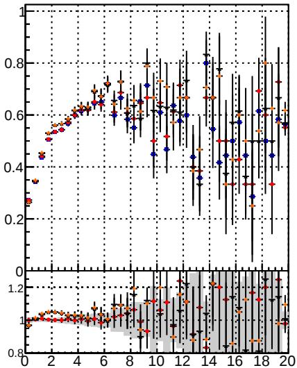
Fake rate vs. BQM noMS PLMS PixelLessOrIDBQM mod MS
