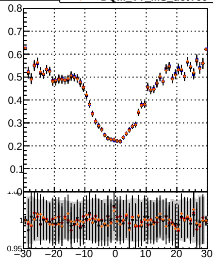
Fake rate vs v Legend: BQM TT MS detT (blue squares) BQM TT MS detT1 (red circles) BQM TT MS detT09 (orange triangles) BQM TT MS detT109 (black crosses)
