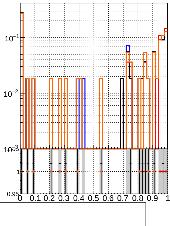
RecoPVAssoc2GenPVNotMatched_missing
