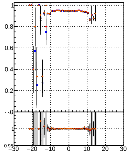
Fake rate vs v — DOM TT MS detT — DOM TT MS detT — DOM TT MS detT
