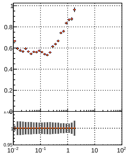
Legend: - \bullet BQM TT MS detT - \bullet BQM TT MS detT1 - \bullet BQM TT MS detT09
