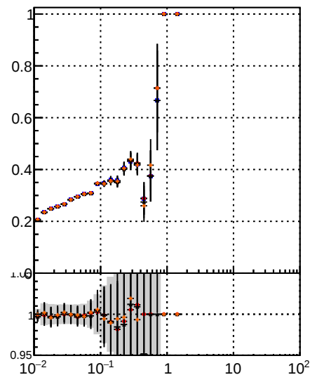
Legend for Fake rate vs v: DOM TT MS detT DOM TT MS detL1 DOM TT MS det09
