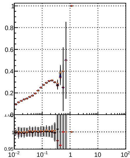
Fake rate vs v BQM detT MS detT BQM detT1 MS detT1 BQM detT09 MS detT09
