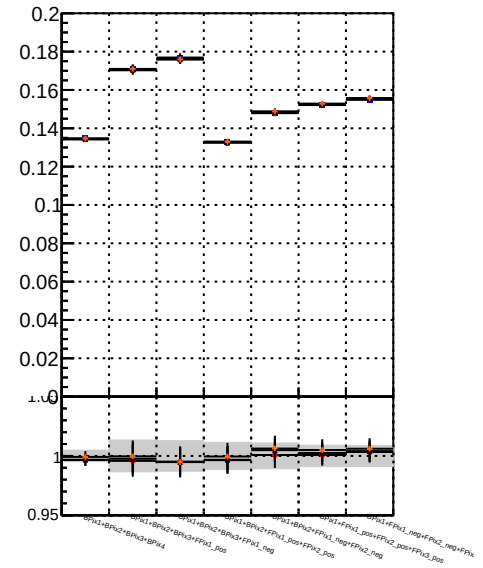
Fake rate vs. BSM MS det1 BSM MS det109
