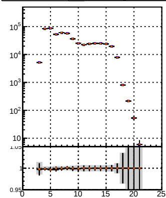
N of reco track vs hit DQM TT MS DQM TT MS detT09 detT09 detT09
