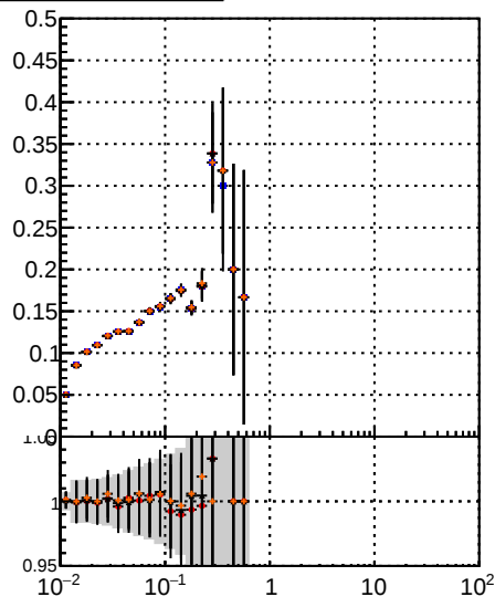
Fake rate vs \sqrt{s} BQM TT MS detT BQM TT MS detL1 BQM TT MS detT09
