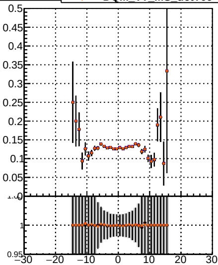
Fake rate vs v_z Legend: DOM TT MS detT DOM TT MS detT1 DOM TT MS detT09
