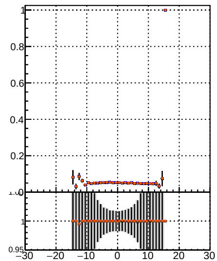
Fake rate vs d BSM \mu\mu MS det1 BSM \mu\mu MS det109
