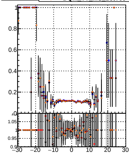
Fake rate vs \nu DOM TT MS detT DOM TT MS detT1 DOM TT MS detT109
