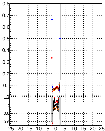
Fake rate vs d BQM det1 MS det1 BQM det2 MS det2
