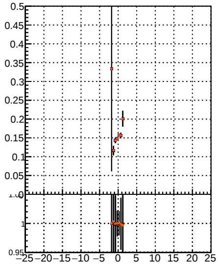
Fake rate vs d BQM MS det1 MS det109 MS det11 BQM MS det1 MS det109 MS det11
