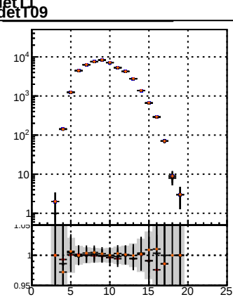
N of associated (recoToSim) tracks vs pixelayer
