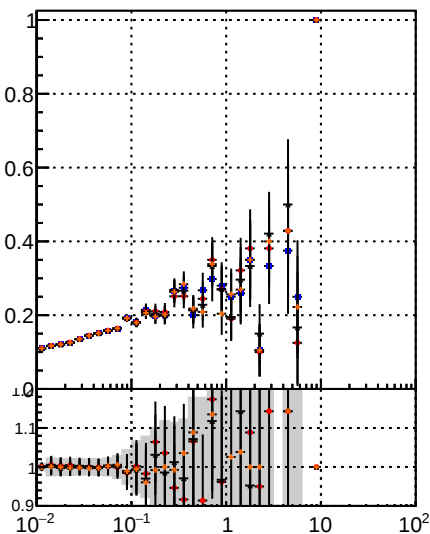
Fake rate vs v Legend: MS (blue squares), MS-detT (red circles), MS-detT1 (orange triangles) MS (blue squares), MS-detT (red circles), MS-detT1 (orange triangles)
