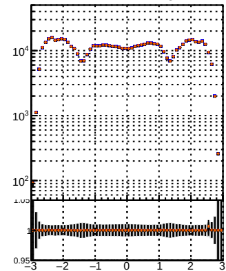
N of reco track vs \eta BQM TT MS delT 1 BQM TT MS delT 1 BQM TT MS delT 1 BQM TT MS delT 1
