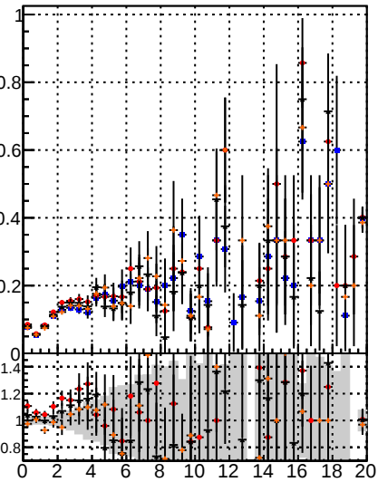
Fake rate vs. Blue circle BQM MS det1 Red circle MS det109
