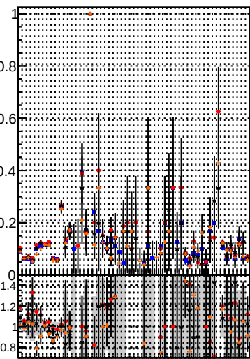
Fake rate vs. Blue circle BQM MS det1 Red circle MS det109
