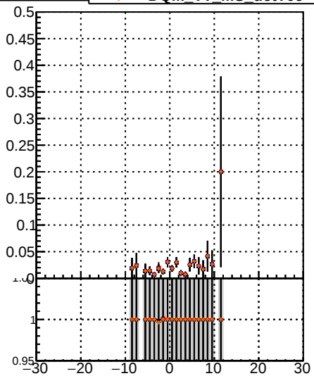
Fake rate vs v_{\text{top}} Legend: \text{DOM TT MS detT} , \text{DOM TT MS detT1} , \text{DOM TT MS detT09}
