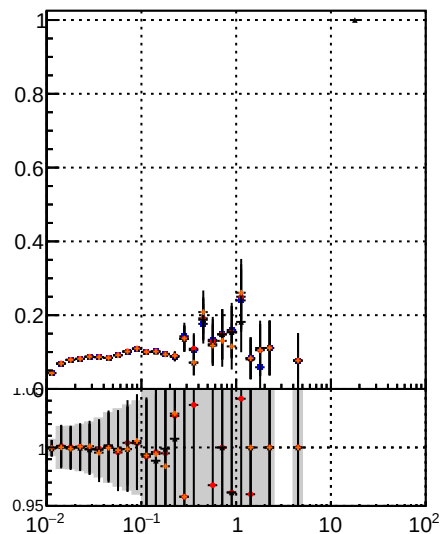
Fake rate vs \nu BQM TT MS detT BQM TT MS detT09
