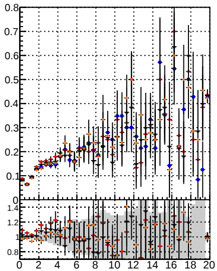
Fake rate vs. BSM MS det1 det109
