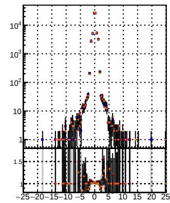
N of reco track vs dxy(PV) N of associated (recoToSim) tracks vs dxy(PV) N of associated (recoToSim) loopier tracks vs dxy(PV)
