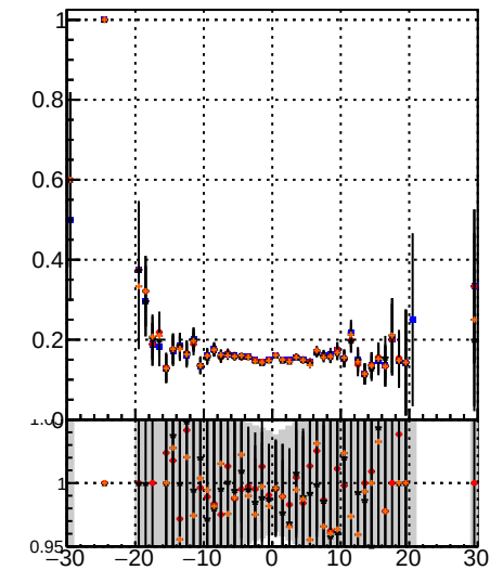
Fake rate vs v DOM TT MS detT DOM TT MS detT1 DOM TT MS detT09
